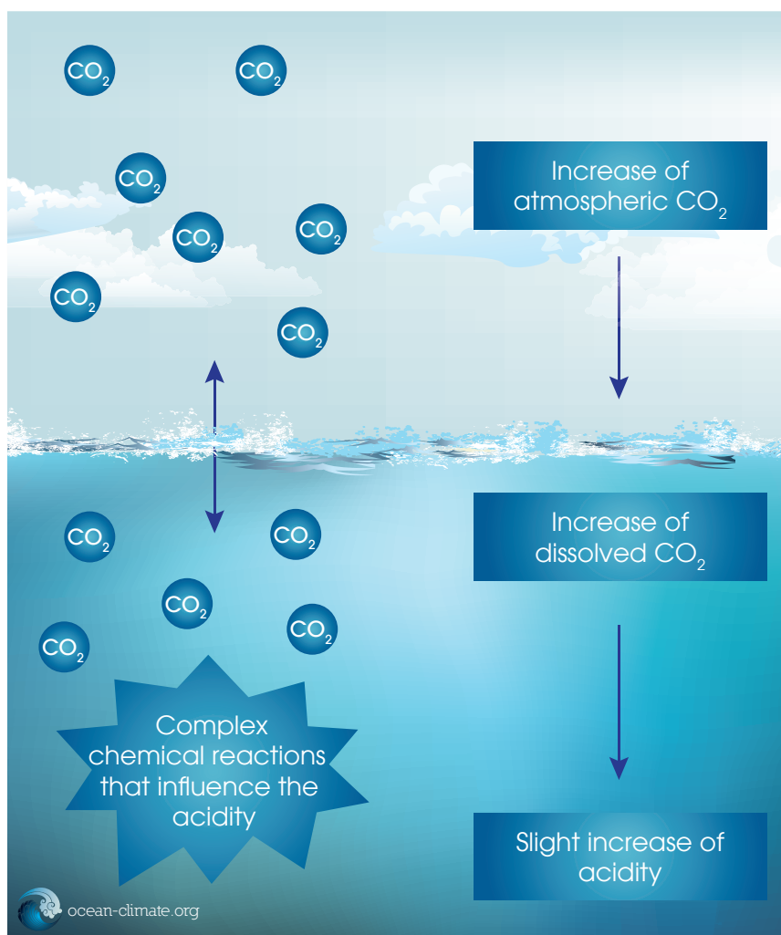
Simplified mechanism of ocean acidification
